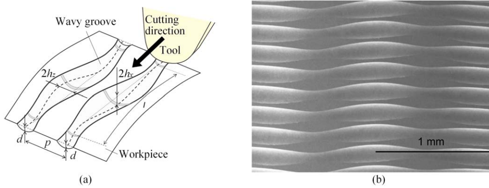
Figure 9. Slow-tool-servo turning for two-directional wavy microgrooves. Reproduced with permission from [105].
