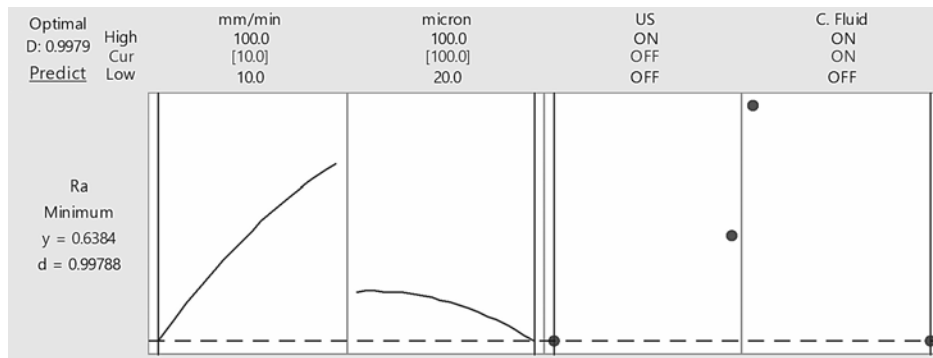
Figure 17 Optimisation plot for Ra
