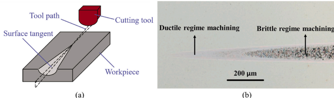
Fig. 5. Taper cutting test. (a) Schematic illustration [2]. (b) Surface topography of the groove on monocrystalline Ge showing the transition of cutting mode [102].
