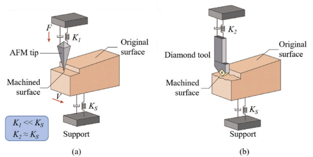
Fig. 24. Schematics of two nanometric cutting approaches [6]. (a) Force control in TBNC. (b) Motion control in diamond tool-based nanometric cutting.
