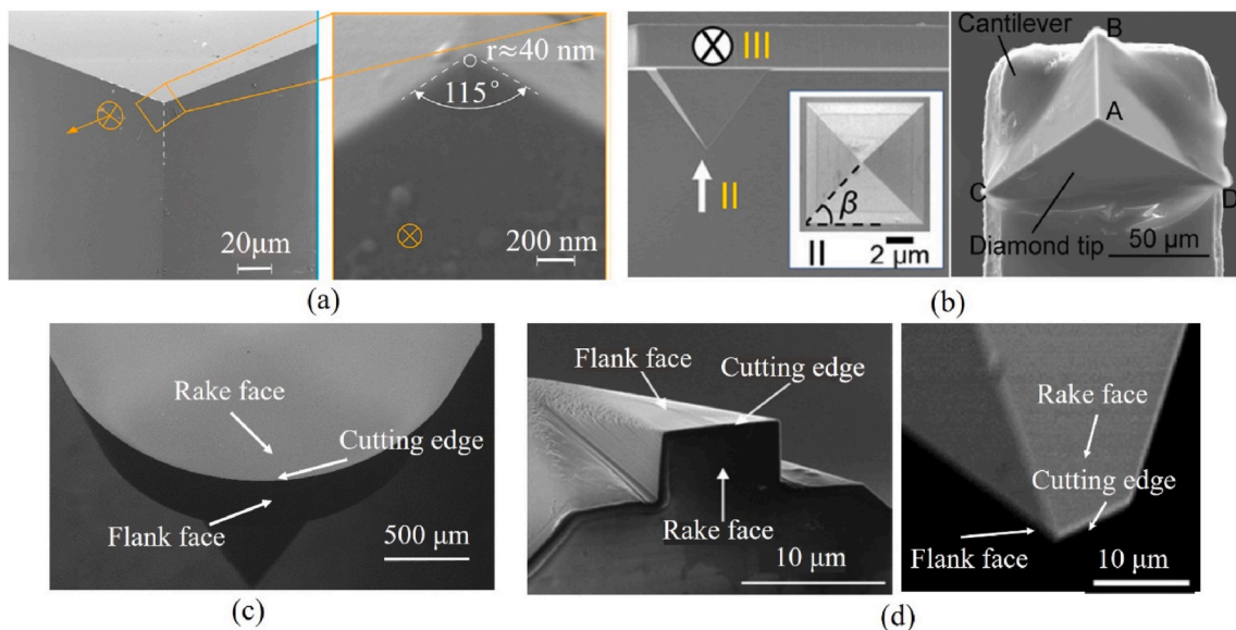
Fig. 3. Diamond tools used in nanometric cutting experiments. (a) Berkovich indenter for nanoscratching [75]. (b) AFM diamond tip with pyramid shape [76, 77]. (c) Commercial diamond lathe tool with a round tool nose for SPDT (See Fig. 19). (d) Customized diamond tool with straight edge for orthogonal cutting [78,79].
