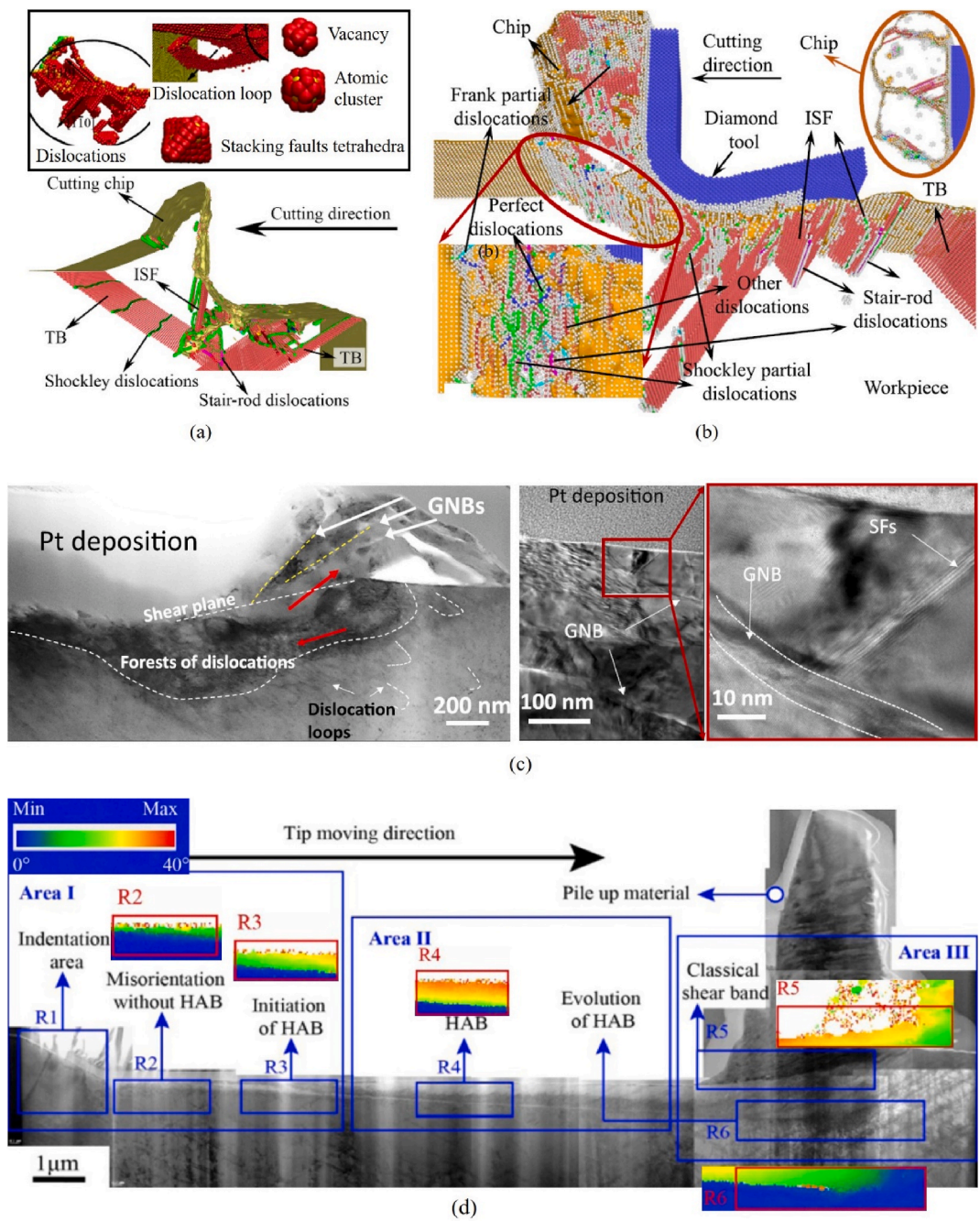
Fig. 9. Structural deformation during the nanometric cutting on metals. (a) MD simulation of microstructure evolution of monocrystalline Cu [31,144]; (b) MD simulation snapshot of microstructure evolution of monocrystalline Al [34]; (c) TEM image of microstructural change in sub-surface areas after AFM-tip based nanoscratching in monocrystalline Cu [131]; (d) TEM image and misorientation map of various crystal structures in subsurface areas from orthogonal cutting experiment with a straight-line-edge tool on a single grain of Ni-based superalloy [78].
