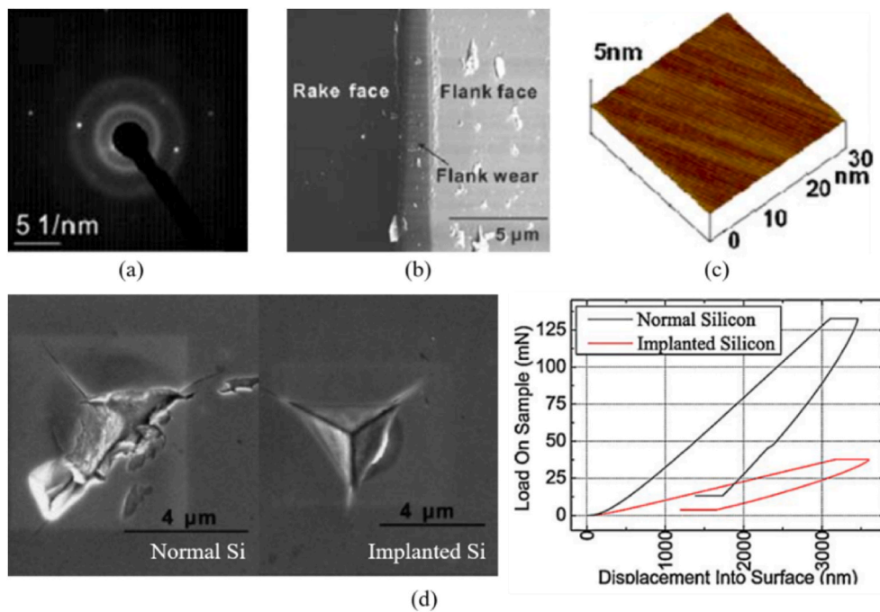
Fig. 15. Improving the machinability of monocrystalline Si by F ion implantation. (a) Electron diffraction pattern of the modified layer. (b) Tool edge after cutting on implanted Si (UCT: 30 nm). (c) Machined surface topography of implanted Si. (d) Nanoindentation marks and load-displacement curves for normal and implanted Si [141].
