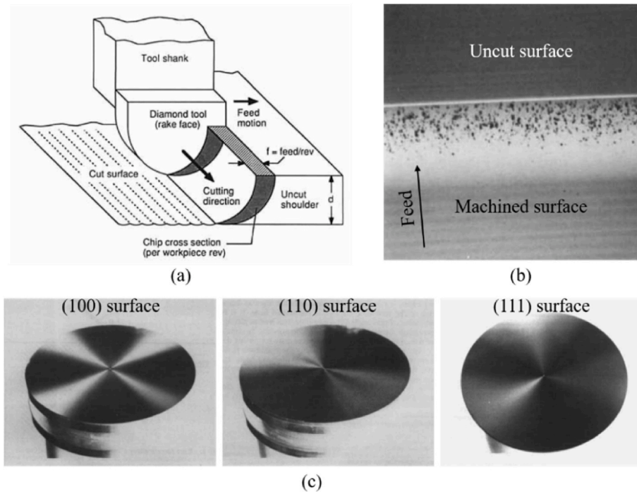
Fig. 19. Investigation of nanometric cutting by single-point diamond turning. (a) Schematic illustration of turning process [160]. (b) Shoulder cutting surface [231]. (c) Pits distribution on diamond-turned Ge with various surface orientations [232].
