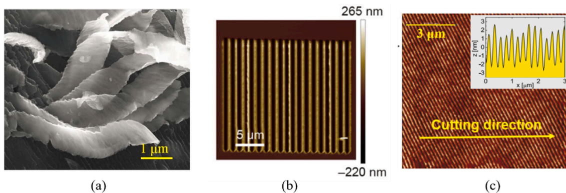
Fig. 25. Characterization of TBNC. (a) Chip of Al alloy. UCT: 270–370 nm, tip radius: 110 nm [259]. (b) Periodic structure formed by pile-up [260]. (c) Formation of nanoripples due to the torsion effect of cantilever [262].
