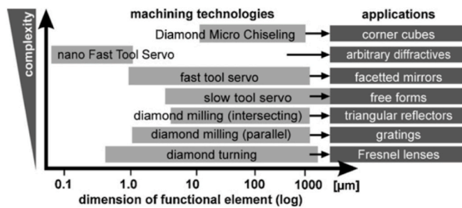
Fig. 23. Machining complexity of surfaces with different functional dimensions [249].
