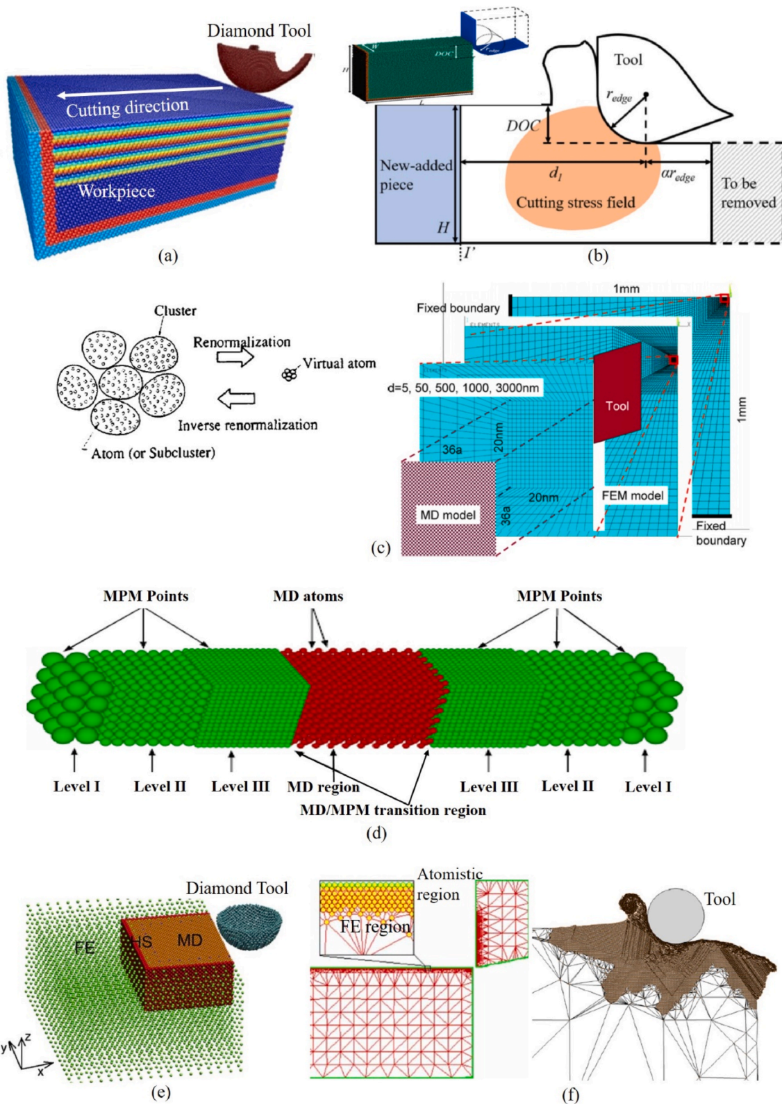
Fig. 2. Numerical simulation models. (a) 3D conventional MD model of nanometric cutting [46]; (b) Dynamic modelling of MD model in nanometric cutting [48]; (c) RGMD model of nanometric cutting [66,68]; (d) MPM-MD model of workpiece in tensile test [69]; (e) MD-FEM model of nanometric cutting using an overlapped handshake region [71]; (f) QC model of nanometric cutting [72,73].
