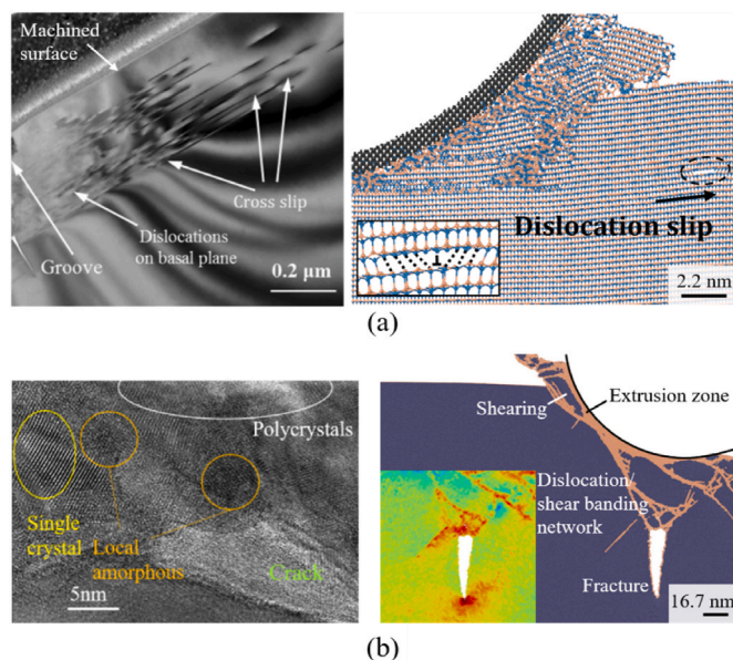
Fig. 12. Comparison between MD simulations and TEM observations. (a) Basal dislocation slips in SiC [65,164]. (b) Subsurface of GaAs (TEM) and Ge (MD) with similar lattice structure [48,52]. The machined surface of GaAs locates in the upper left direction and the local view of simulation is the first principal stress distribution near the crack.
