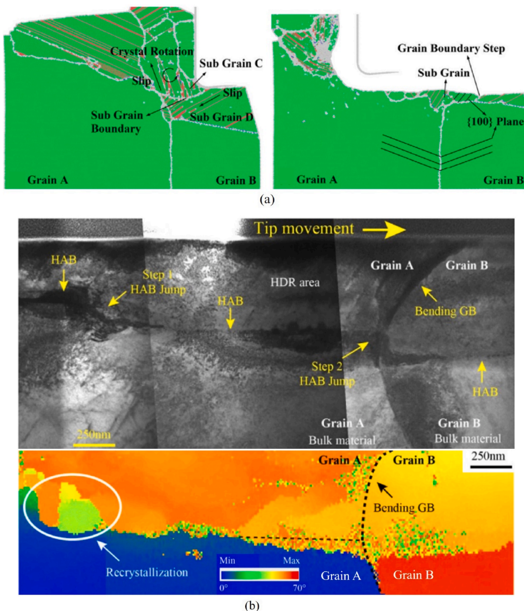
Fig. 10. Dislocations in nanometric cutting. (a) MD simulation snapshot of microstructure evolution of polycrystalline Cu (UCT: 14.46 nm) [150]; (b) TEM image and misorientation map of structural variation in subsurface areas from orthogonal cutting across the GB of Ni-based superalloy [78].
