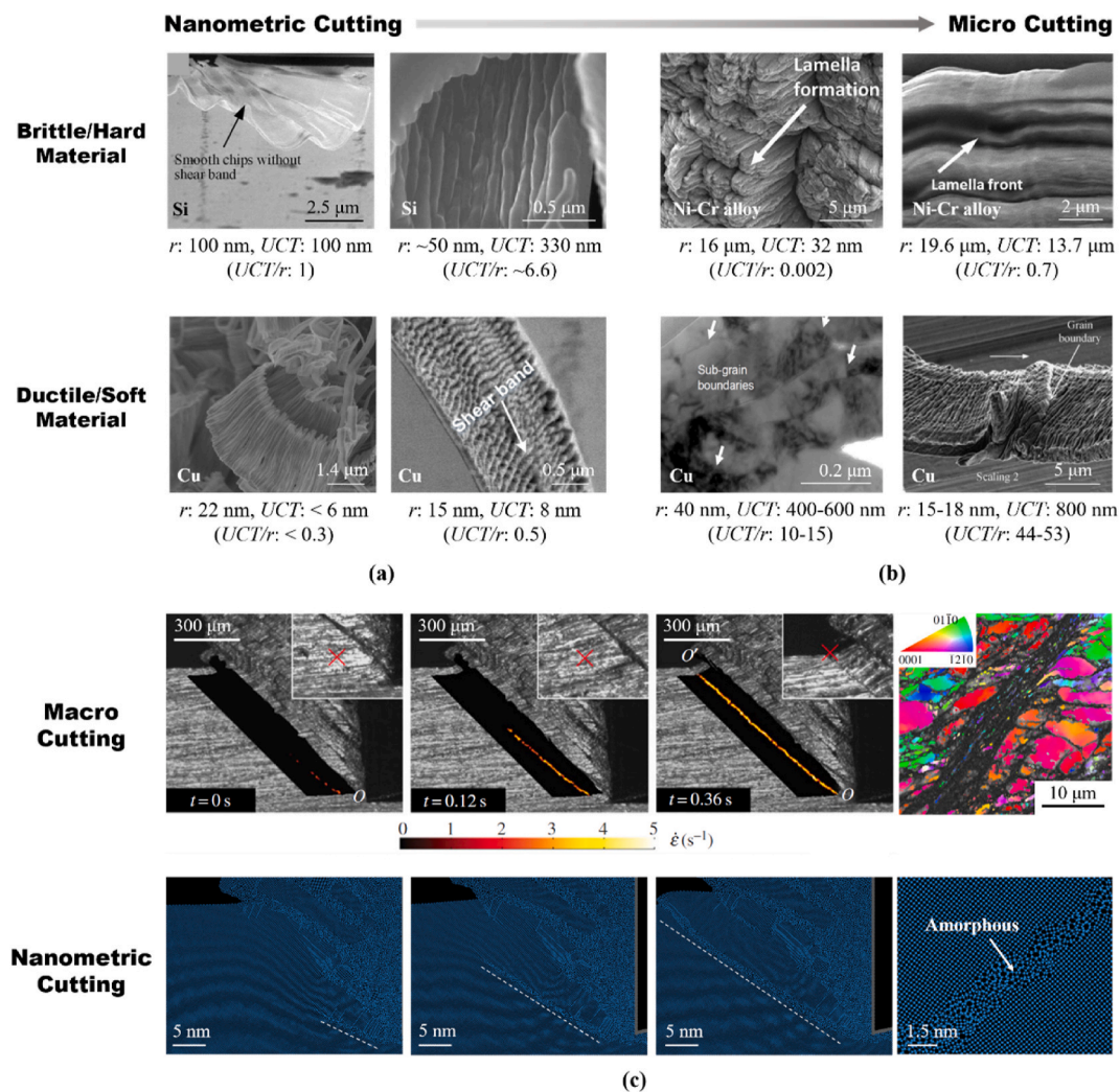
Fig. 8. Comparison of chip formation at different scales. Chip morphology of two kinds of materials from (a) nanometric [95,105,126,128] to (b) micro scale [129–131]. ( r : edge radius) (c) Shear banding process. Up: High-speed camera images of cutting on cold-worked brass (UCT: 600 \mu\text{m} ) and EBSD map of the shear band in titanium alloy chip (UCT: 125 \mu\text{m} ). (Edge radius: 10 \mu\text{m} ) [132] Below: MD simulation on Si using a sharp tip (UCT: 20 nm).
