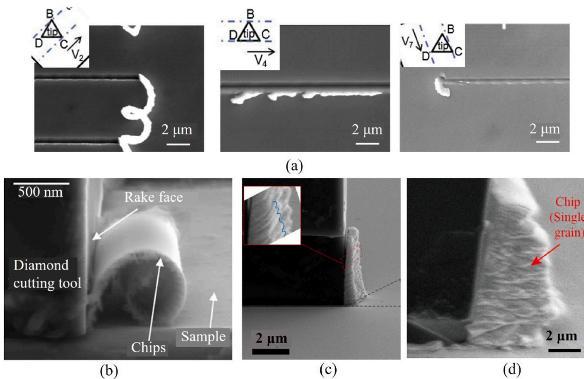
Fig. 4. Chip and pile-up formation in different nanometric cutting experiments. (a) SEM image of machined surfaces with AFM pyramid tip along different scratching directions, UCT <200 nm [77]; (b)–(d) In-situ SEM observation of chip formation in orthogonal cutting: (b) monocrystalline Cu, UCT < 100 nm, cutting length is 7 μm and cutting speed is 23.5 nm/s [79]; (c) monocrystalline Cu, UCT is 500 nm, cutting length is 7 μm and cutting speed is 70 nm/s [93]; (d) Ni-based superalloy, UCT is 1 μm, cutting length is 12 μm and cutting speed is 2 μm/s [78].
