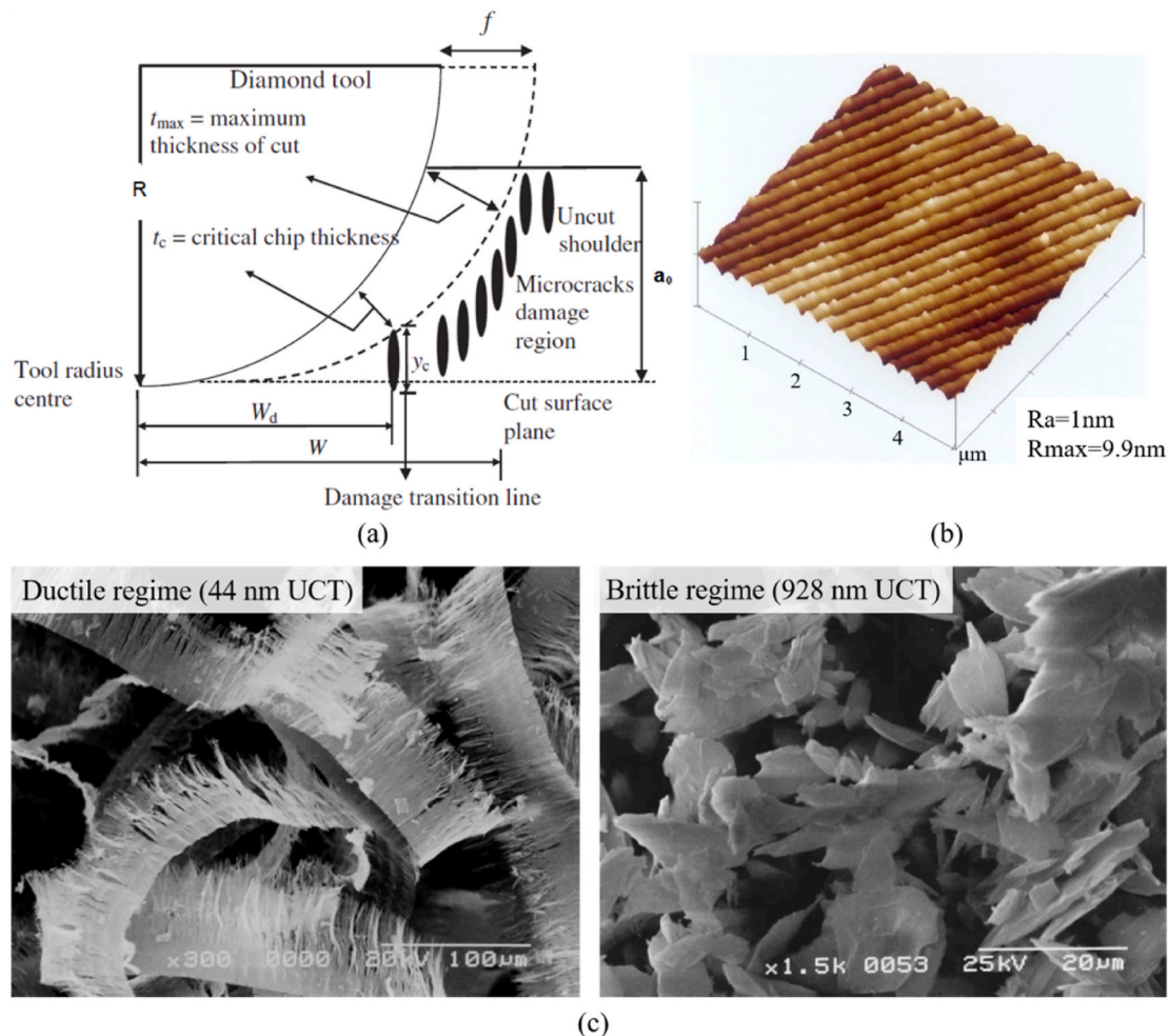
Fig. 11. Machining of brittle materials in ductile and brittle regimes. (a) Schematic model of material removal in diamond turning [160]. (b) Si surface with a Ra of 1 nm by ductile-regime cutting [2]. (c) Si chip morphologies in various cutting regimes [161].
