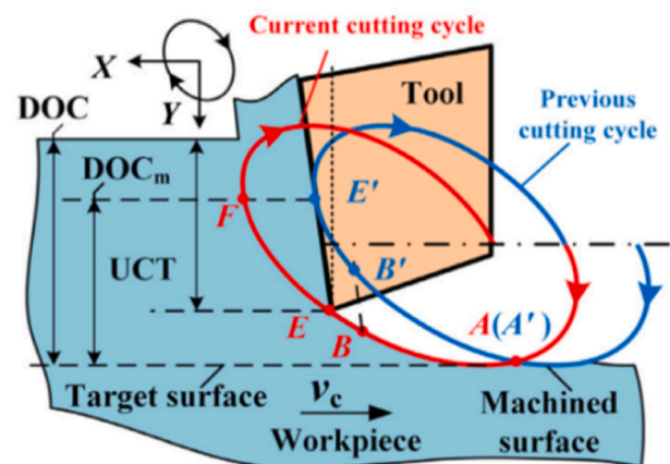
Fig. 18. Geometric model of elliptical UVAC. The material is intermittently removed in each vibration cycle, and the overlapped tool path makes a nanometric UCT [207]. (A/A': start contacting, E: rapid increase in UCT, F/E': disengage).
