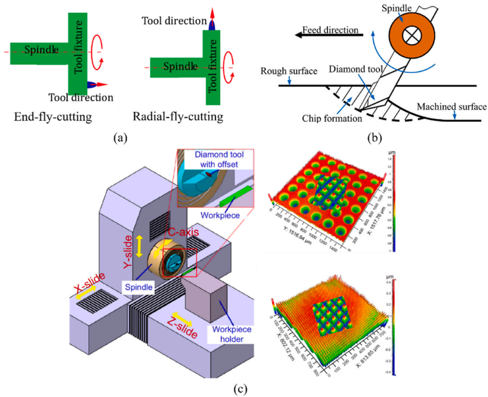
Fig. 21. Diamond fly cutting. (a) Setup of two machining modes [240]. (b) Material removal in (radial) fly-cutting [243]. (c) Micro–nano hierarchical structures machined by end-fly-cutting-servo method [245].
