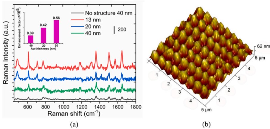
Fig. 27. Surface-enhanced Raman substrate [271]. (a) Raman spectrum from substrates with and without array structure. (b) AFM image of the nanodots array substrate deposited with 40 nm Au film.
