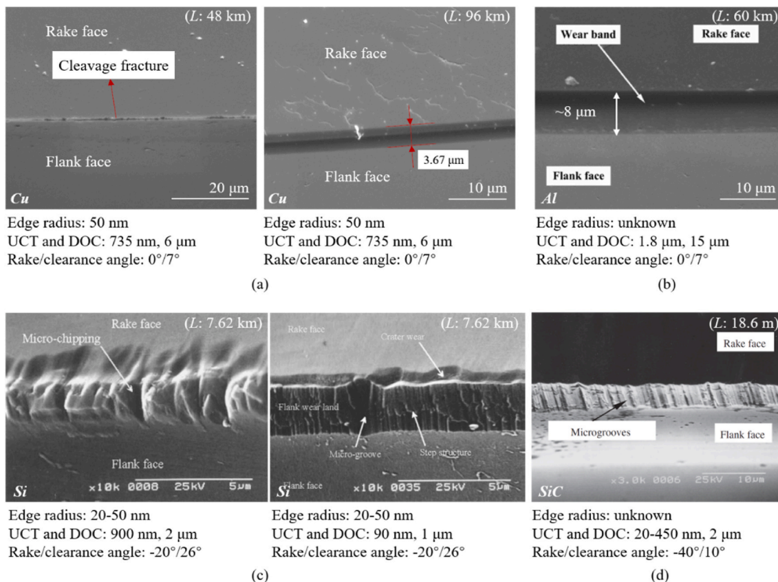
Fig. 13. Tool edge wear of cutting on typical materials with cutting length (L) in each subfigure. (a) Cu [176], (b) Al [178], (c) Si (left: ductile-regime, right: brittle-regime) [12], (d) SiC [181].
