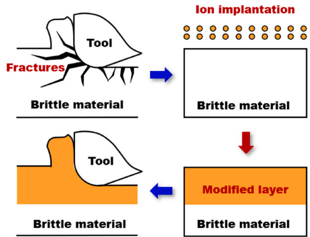
Fig. 14. Illustration of NiIM. Formation of the modified layer with plenty of lattice defects is critical for depressing fractures during the cutting.
