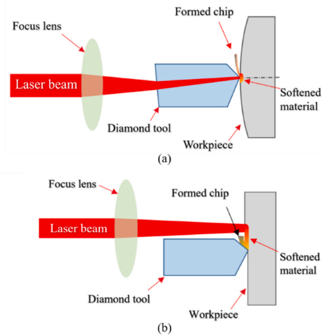
Fig. 17. Two types of LAC [194]. (a) Laser in-process-heat-assisted cutting. (b) Laser pre-heat-assisted cutting.
