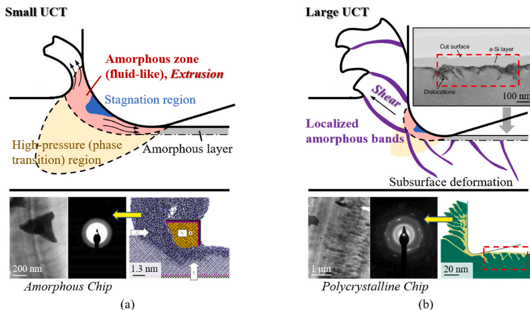
Fig. 7. Schematic illustration of nanometric cutting model with evidences from experiments and simulations [7,123,125]. (a) Cutting under small UCT is dominated by extrusion. The chip and the machined surface layer are amorphous. (b) Larger UCT results in the coexistence of extrusion and shearing. Polycrystalline structure is observed in the chip and the machined surface.
