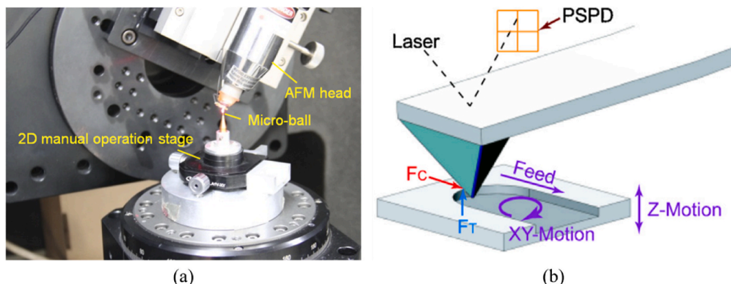
Fig. 26. Realization of TBNC. (a) Five-axis AFM-based machining system [265]. (b) Vibration-assisted nanometric cutting method based on an AFM [266].
