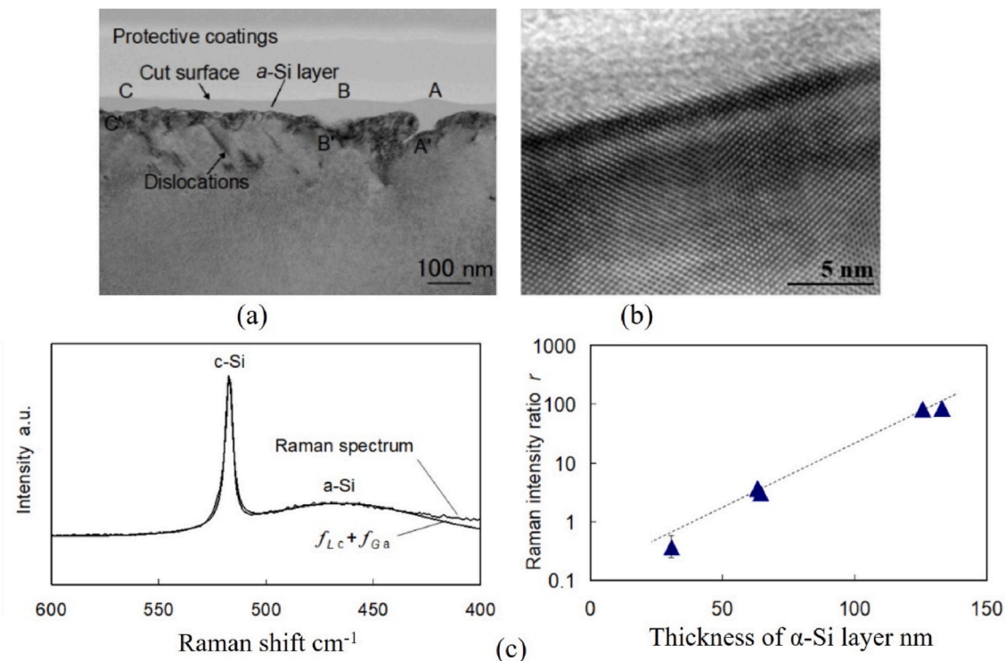
Fig. 6. Subsurface information in nanometric cutting revealed by TEM and Raman spectra. (a) Subsurface deformation of machined Si [7]. (b) High-resolution TEM observation of machined Ge surface lattice [3]. (c) Quantitative evaluation of amorphous layer thickness using Raman intensity ratio [115].
