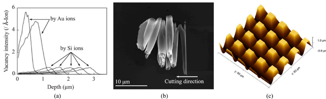
Fig. 16. Surface modification by multi-ion implantation. (a) Vacancy distribution of each individual implantation. (b) Cutting chip morphology indicates a significant enhancement in the workpiece ductility [128]. (c) Microstructure array on the implanted Si machined by fly cutting.
