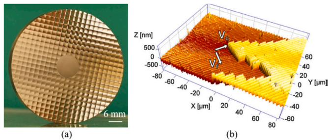
Fig. 20. Array structures machined by FTS. (a) Lens array of beam integrator (UCT: 970 nm) [236]. (b) WLI measurement of submicron structure on nickel silver machined by nano-FTS [233].
