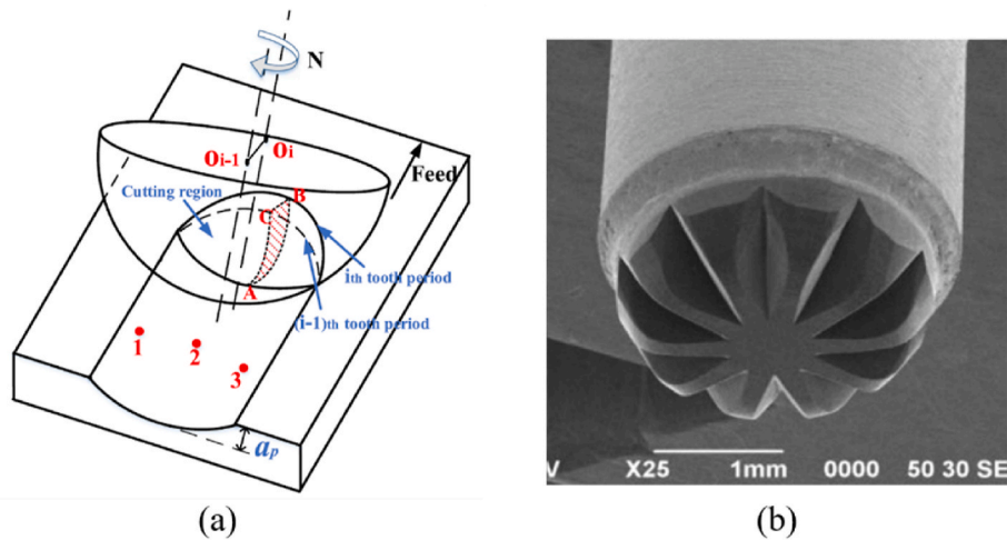
Fig. 22. Diamond milling. (a) Material removal model [247]. (b) Multi-edge milling tool [248].
